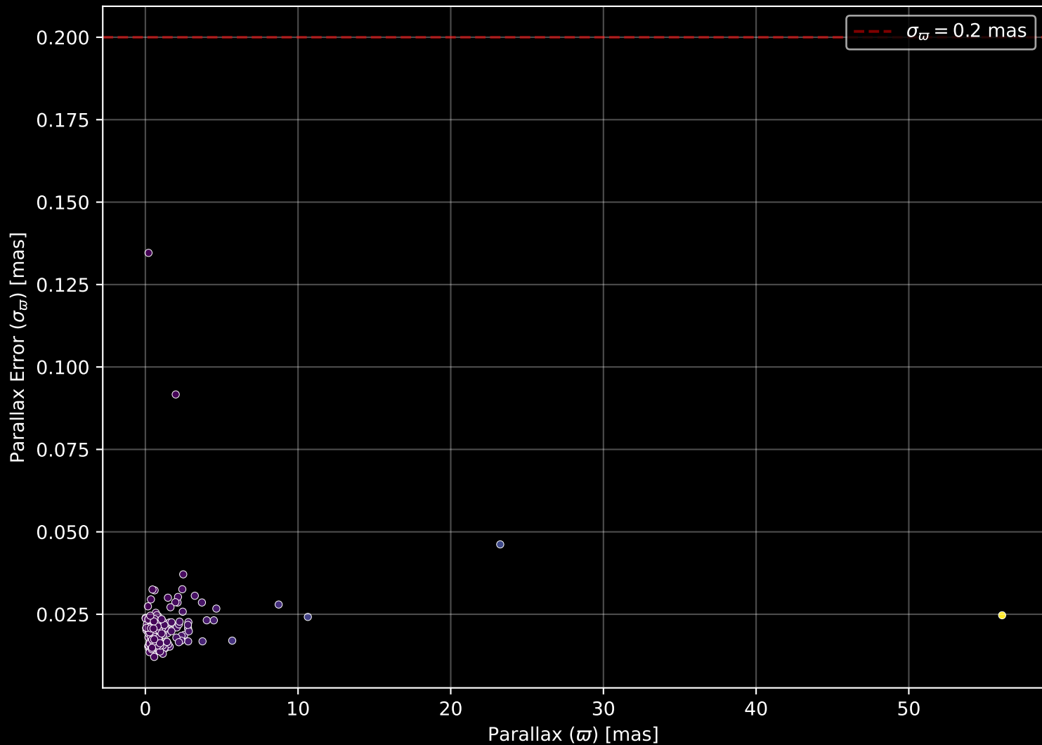
APOGEE DR17 Field: [210+30] Parallax Quality (n= 172)
