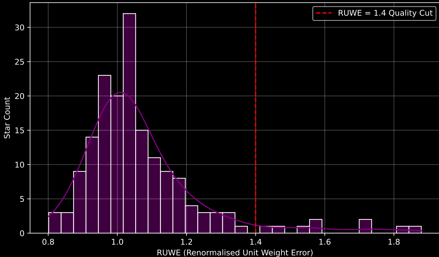
GAPOGEE DR17 Field [210+30] RUWE Distribution (n= 170)
