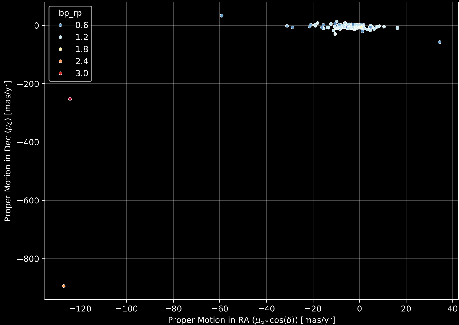
APOGEE DR17 Field: [210+30] Proper Motion Diagram (n= 172)
