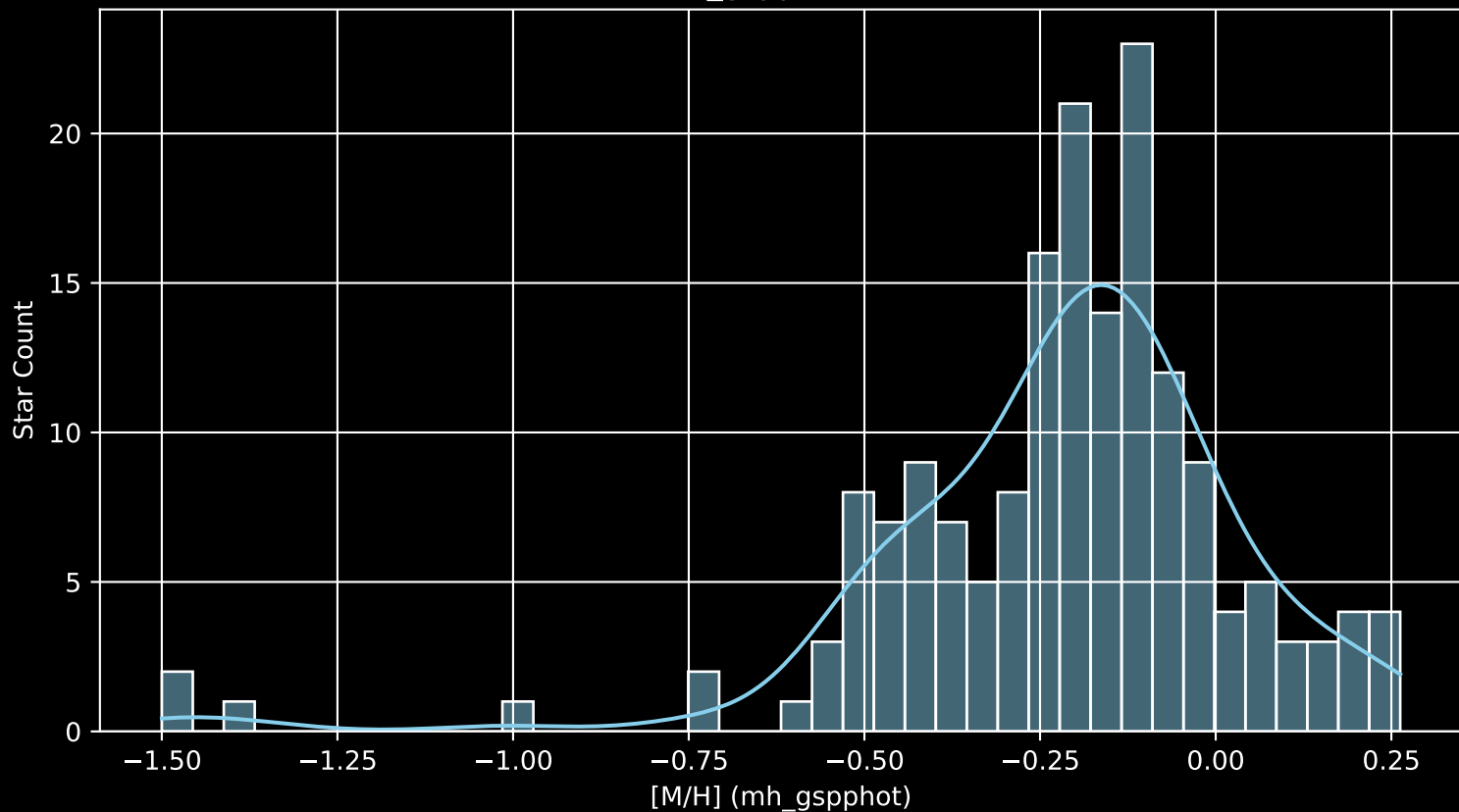
APOGEE DR17 Field: [210+30 [M/H] (mh_gspphot) (n= 172)
