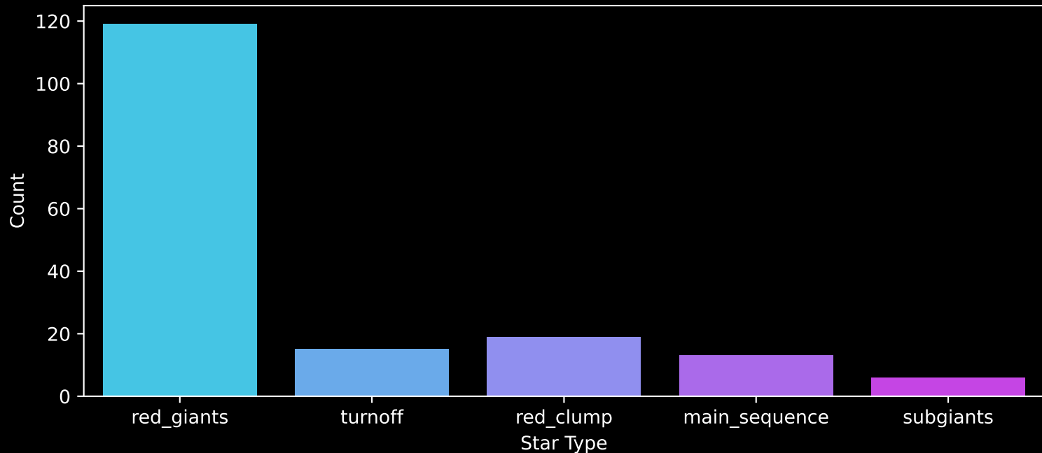
APOGEE DR17 Field: [210+30] Count plot of Star Type
